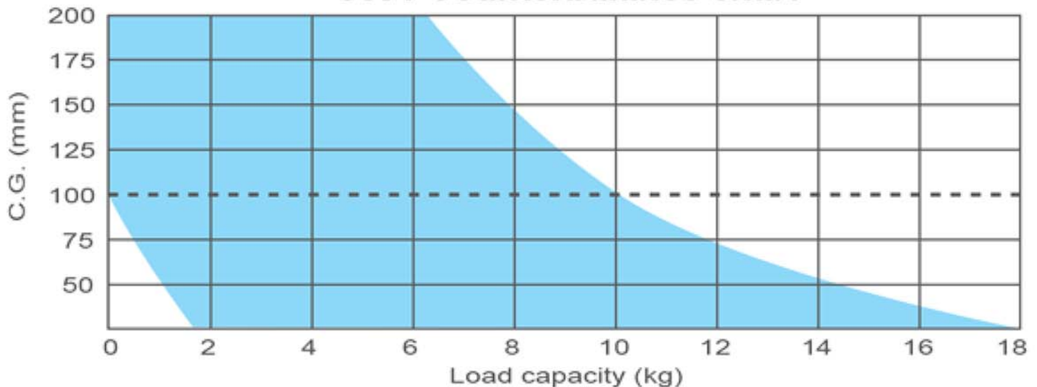
CH4 Counterbalance chart
