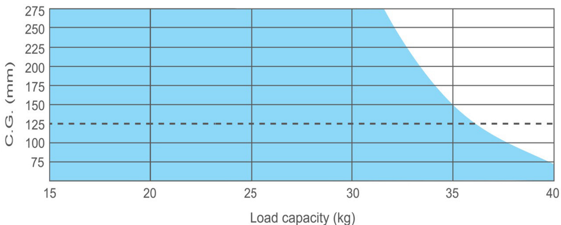
CHX(F) Counterbalance chart
